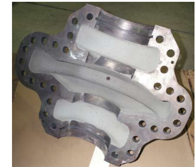
Figure 8. Denise No. 2 horizontal split-case pump – upper half of pump housing after stainless steel plasma coating.
